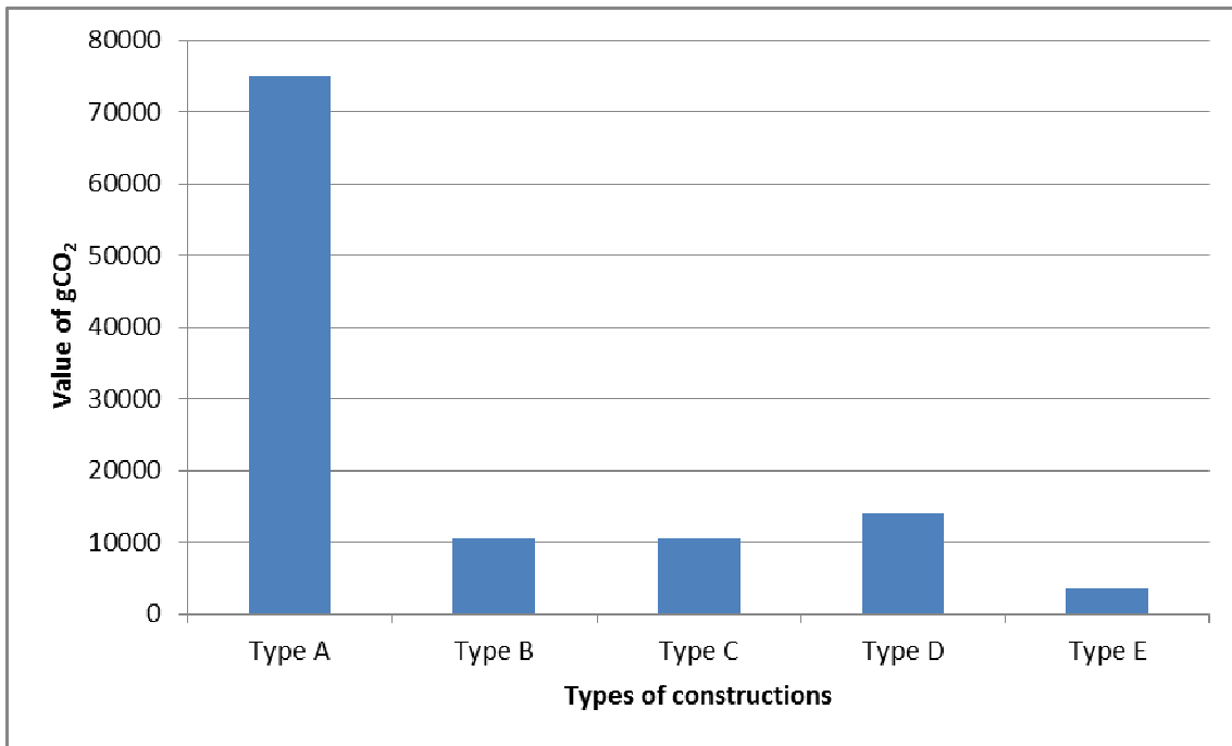
Figure 2. The value g of CO 2 in the extraction and production of raw materials and products of different types of terrace / retaining walls.
