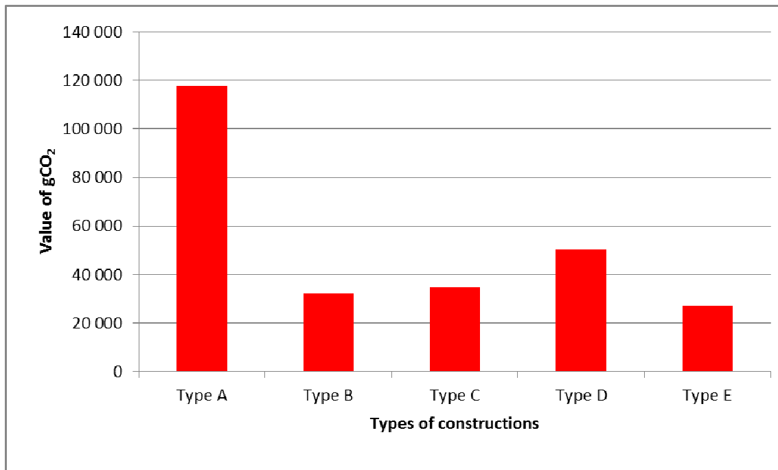
Figure 5. The total value of gCO 2 for all the processes of different types of terrace / retaining walls including earthworks.
